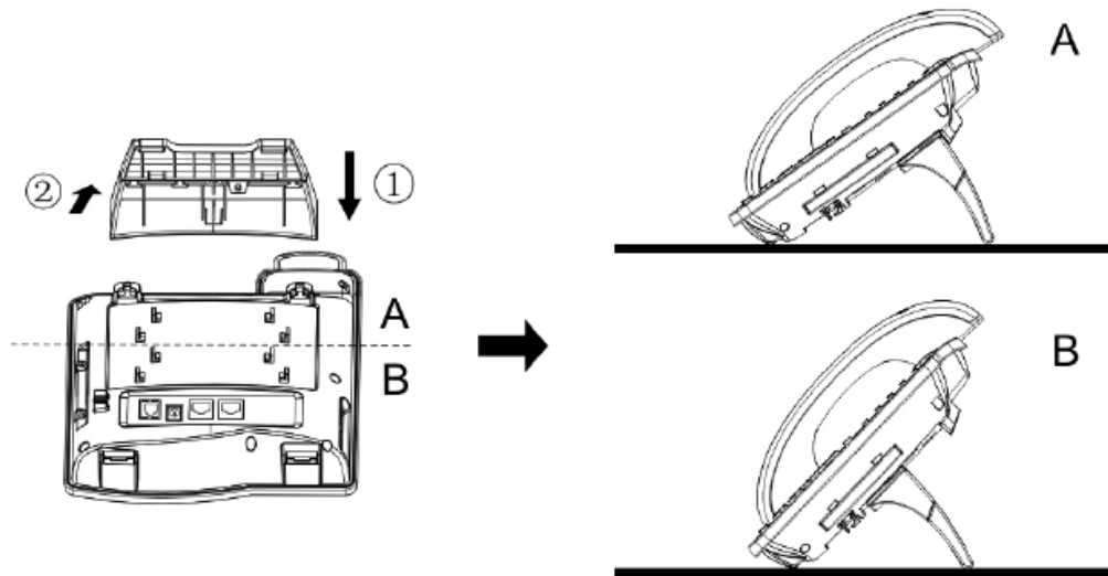
Fig 1. Bracket Installation
