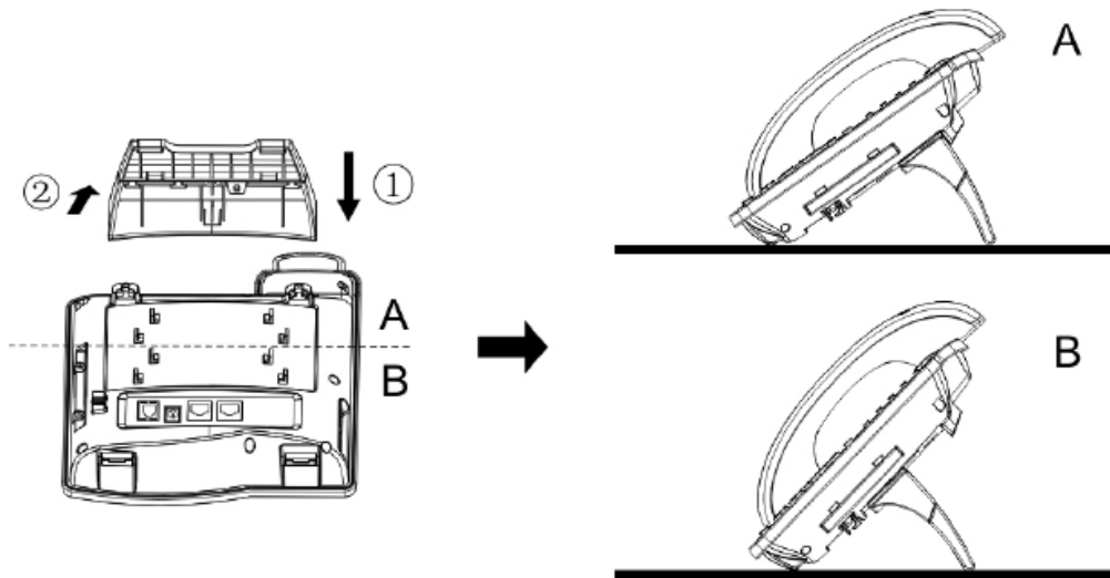
Fig 1. Bracket Installation
